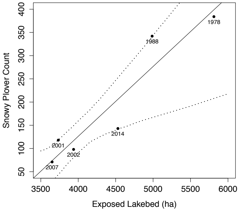
Figure 3. Scatter plot with solid line representing the mean of bootstrapped estimates by ordinary least squares depicting the positive correlation between numbers of Snowy Plovers detected and the extent of exposed lakebed at the time of six surveys at Mono Lake, 1978–2014. Intercept (95% confidence interval) = -475.6 ( -713.5 , -90.3 ), slope coefficient = 0.15 ( 0.05 , 0.21 ), r^2 = 0.89 ( 0.59 , 1.00 ). Dotted lines represent the 95% confidence interval of bootstrapped estimates. Plover counts labeled by year.
