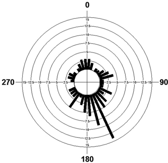
Figure 1. Compass orientation, with respect to the substrate's trunk, of Black-chinned Hummingbird nests in southeast Arizona ( 0^\circ = north). The length of a given bar expresses the number of nests oriented in that direction.
